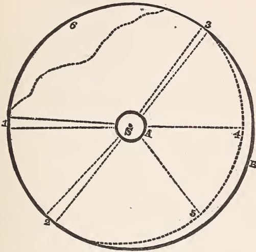
FIG. 5.—THE GALACTIC CLOVEN FLAT RING (PLAN).
